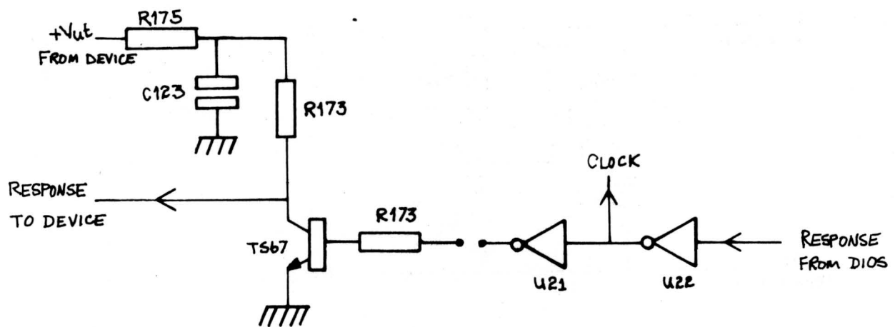
FIGURE 5.12 TRANSMITTER CIRCUIT
