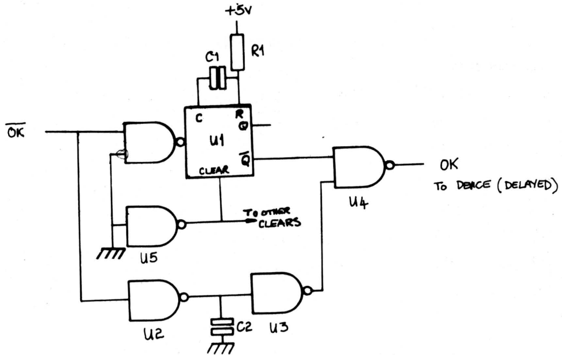
Figure 5.7 Schematic diagram of delay circuit
