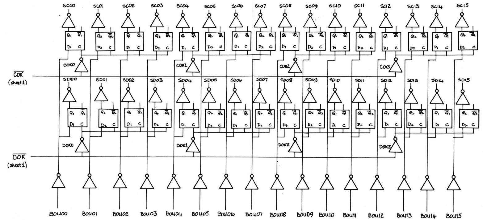
Figure 5.3b DIOC: OUTPUT CHANNELS
