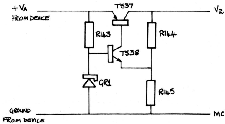
Fig. 5.15 VOLTAGE REGULATOR
