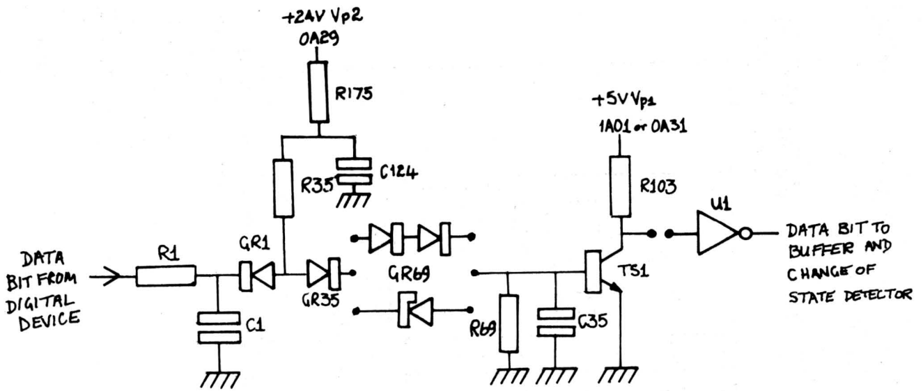
FIGURE 5.9 RECEIVER CIRCUIT
